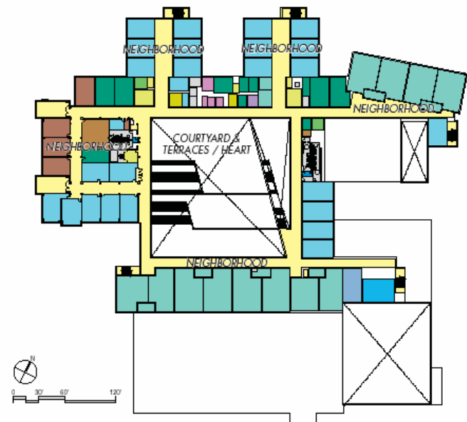
Third Floor Plan, showing academic neighborhoods around the "heart"
