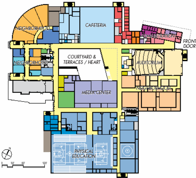
First floor plan organization of a five neighborhood public program around the "heart"
